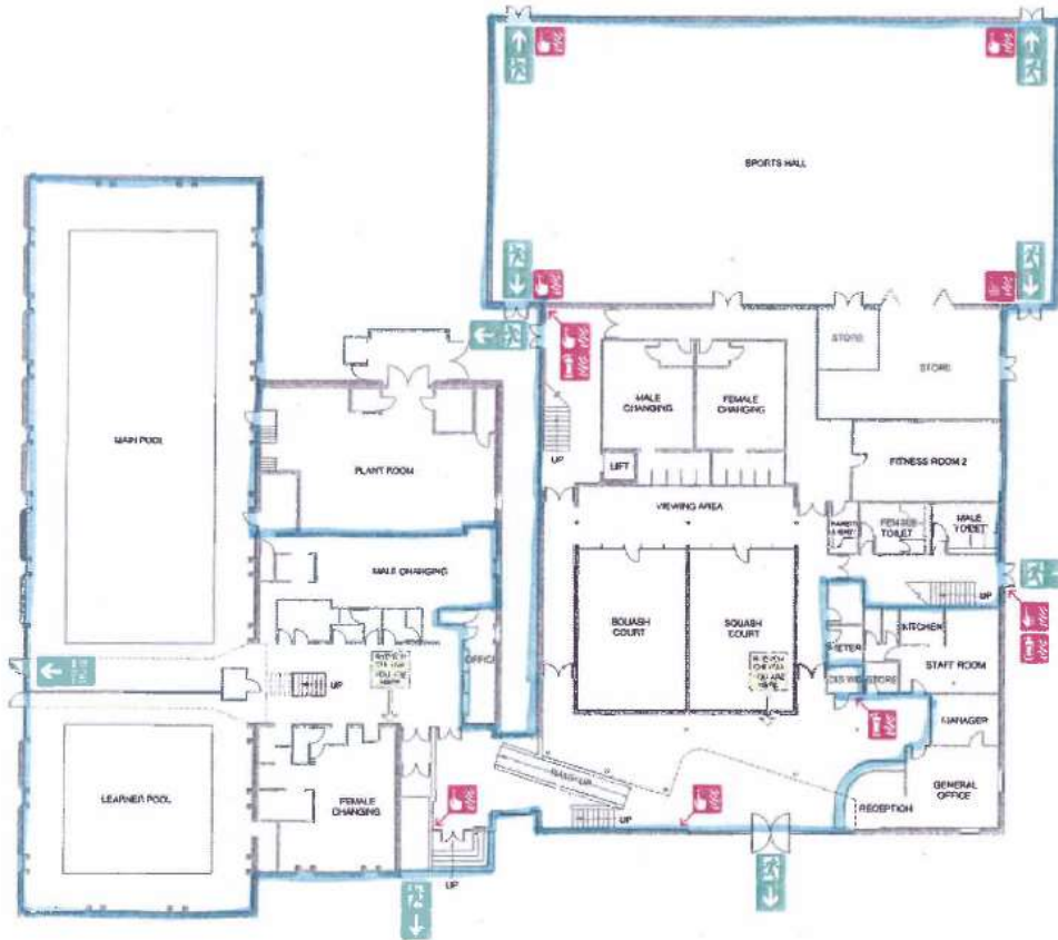
LLAWR GWAELOD ~ GROUND FLOOR
