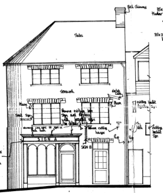
Front Elevation 1:50 Sc
